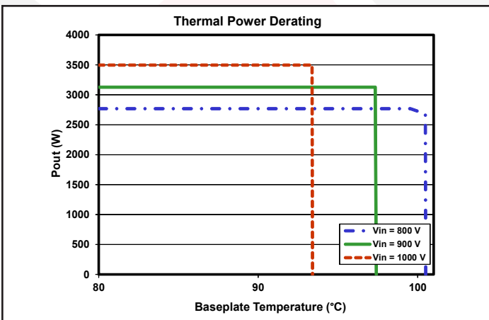
Figure 5: Maximum output power vs. baseplate temperature for minimum, nominal, and maximum input voltage.
