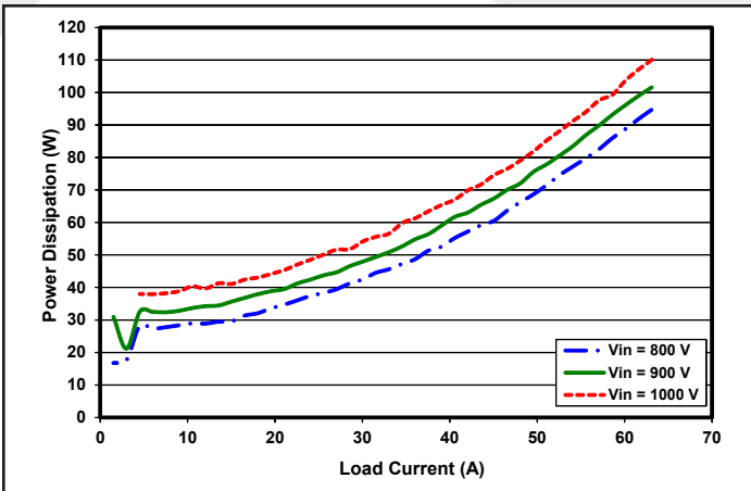
Figure 3: Power dissipation vs. load current for minimum, nominal, and maximum input voltage at T_{CASE}=25\text{ °C} .
